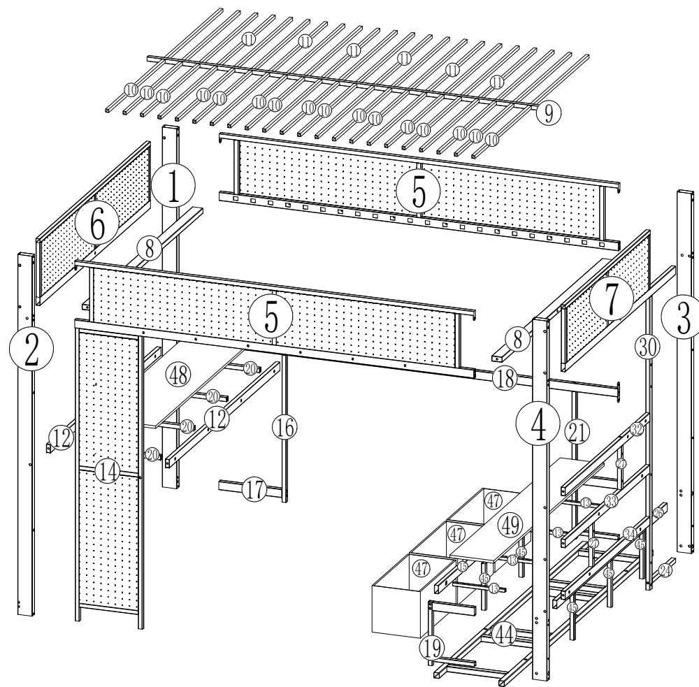
Bed parts view
