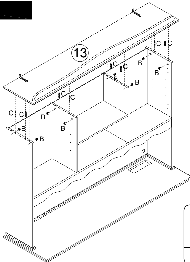
Dowel
