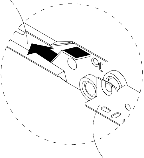
Drawer Slide
